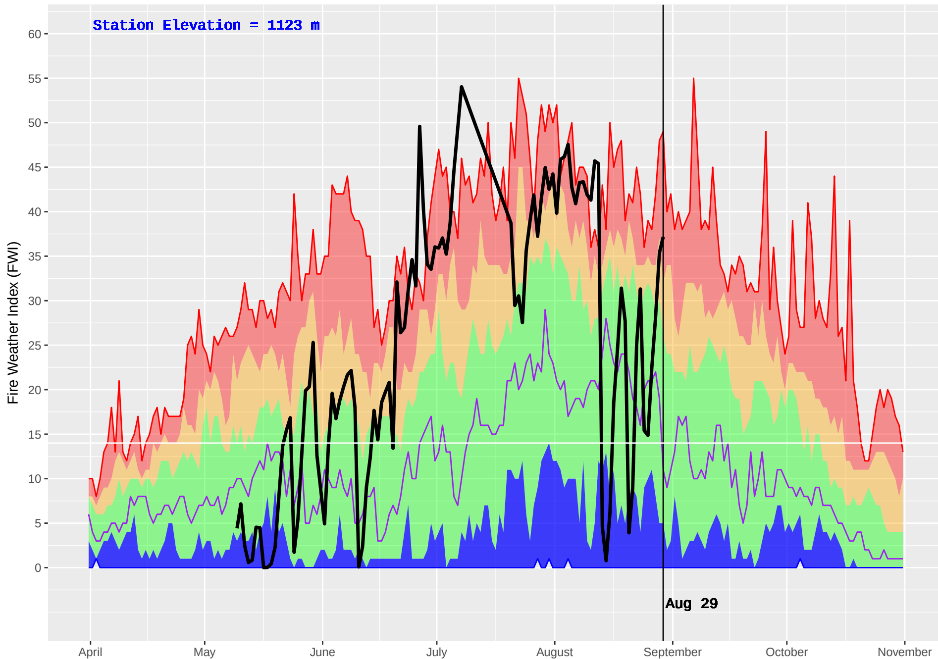
MCLEAN LAKE (311) : Historical (1987–2016) and Current (2017) Noon Fire Weather Index (FWI)
