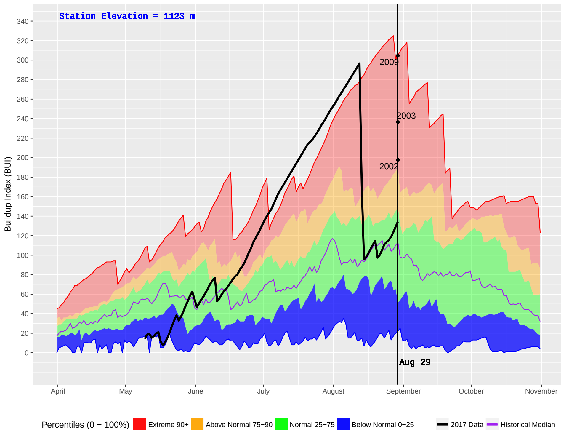
MCLEAN LAKE (311) : Historical (1987–2016) and Current (2017) Noon Buildup Index (BUI)
